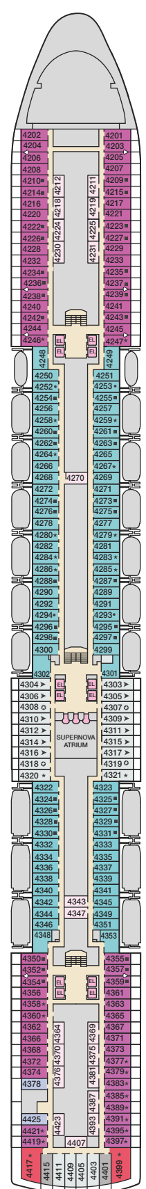
Deck 4
